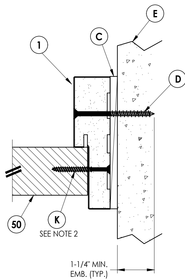
2 HORIZONTAL CROSS SECTION 8 Shown Direct to Masonry Outswing shown (Inswing similar)
