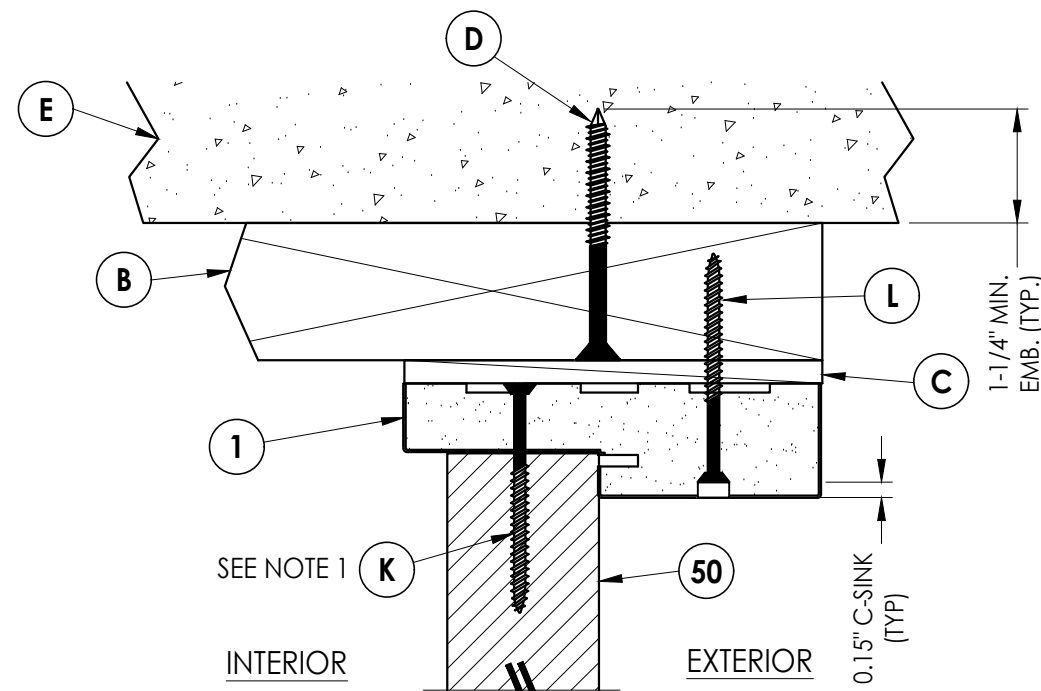
4 VERTICAL CROSS SECTION 6 Outswing shown (Inswing similar)
