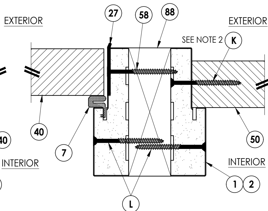
6 HORIZONTAL CROSS SECTION 6 Outswing shown (Inswing similar)
