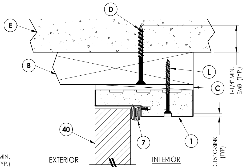
3 VERTICAL CROSS SECTION 6 Outswing shown (Inswing similar)
