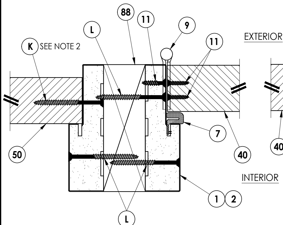
5 HORIZONTAL CROSS SECTION 6 Outswing shown (Inswing similar)
