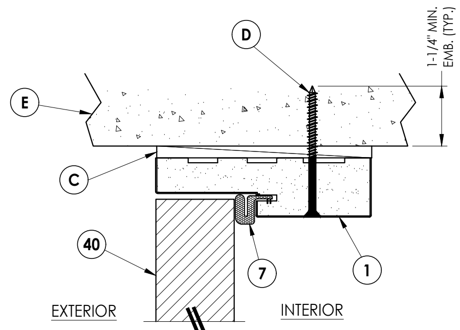
3 VERTICAL CROSS SECTION 8 Shown Direct to Masonry Outswing shown (Inswing similar)
